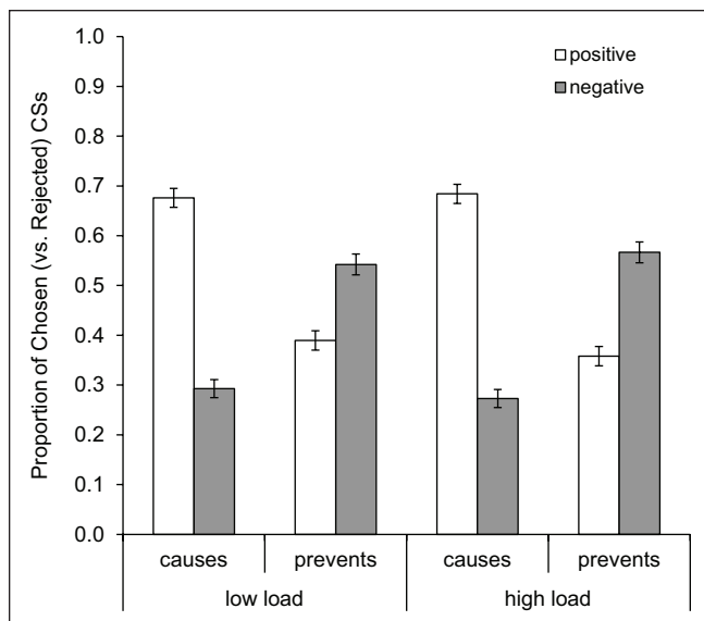
Figure 3. Mean proportions and 95% confidence intervals of choice responses (yes vs. no) as a function of valence of co-occurring stimulus (positive vs. negative), relation to co-occurring stimulus (stimulus causes vs. prevents co-occurring stimulus), and cognitive load (low load vs. high load), combined data from Experiments 1 to 3.
